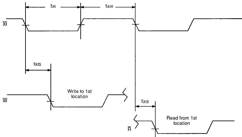
Figure 11. 1st Clock Pulse Delay from \bar{Xl}
