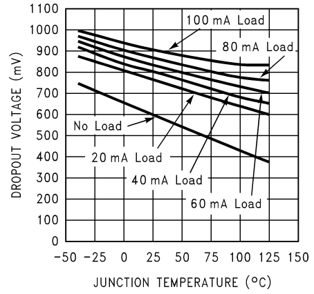
Dropout Voltage vs Junction Temperature
